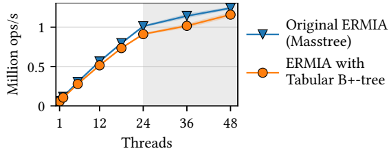
Figure 12: TPC-C throughput with Masstree vs. Tabular B+-tree.
