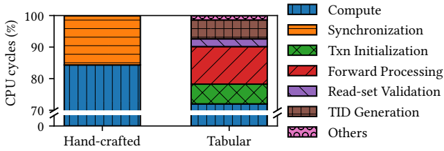
Figure 9: CPU cycle breakdown of Hand-crafted and Tabular B+-trees running the lookup-only workload under 24 threads.
