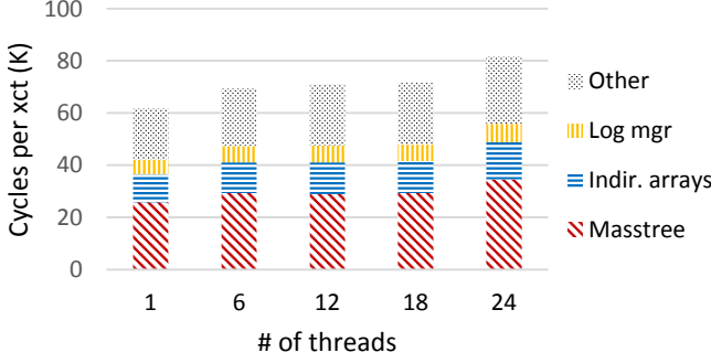
Figure 11: Cycle breakdown of the various components of ERMIA-SI when running an increasing number of threads run TPC-C.
