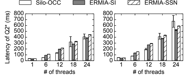
Figure 12: Latency of TPC-CH-Q2* at 60% size (left); 80% size (right), varying the number of threads. Under Silo-OCC, latency fluctuates with larger transaction size and higher concurrency.
