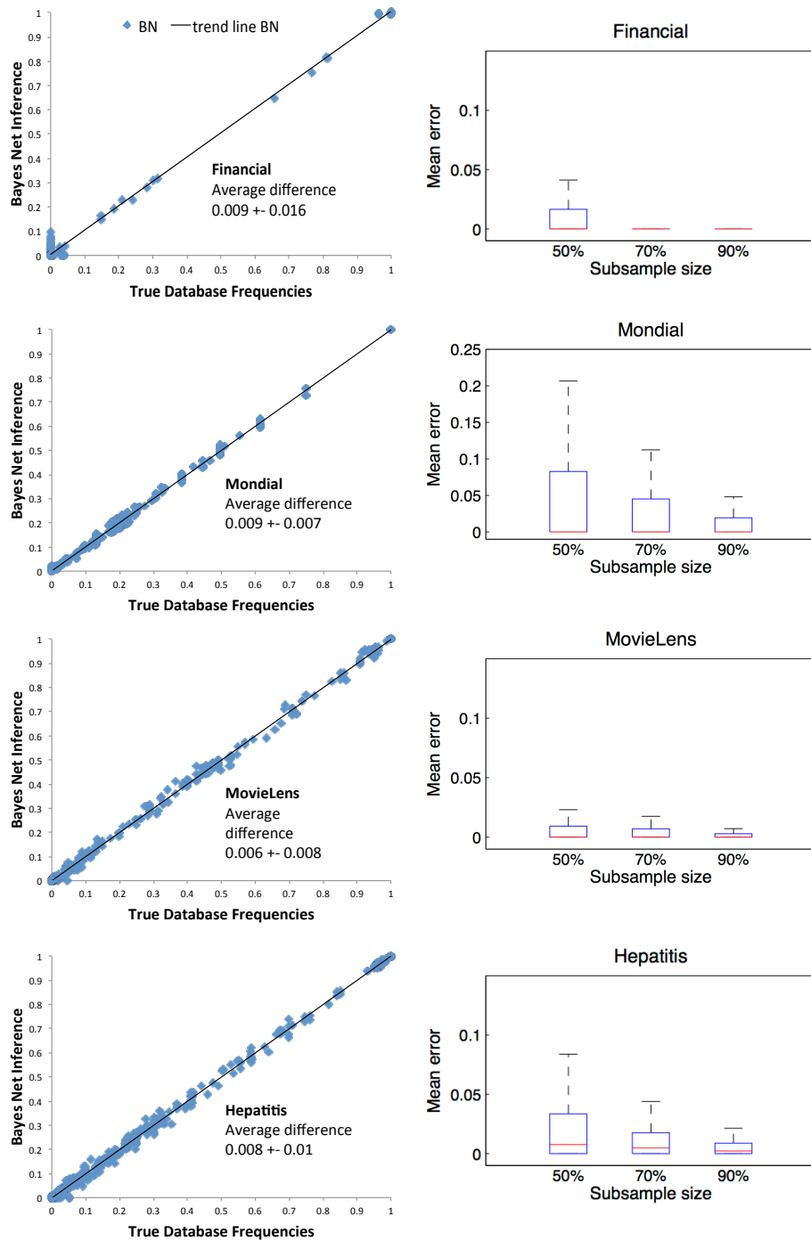
Fig. 5. Left: Query performance (Section 6.3): Estimated vs. true probability, with average error and standard deviation. Number of queries/average inference time per query: Mondial, 506/0.08sec; MovieLens, 546/0.05sec; Hepatitis, 489/0.1sec; Financial, 140/0.02sec. Right: Error (Section 6.4): Absolute difference in estimated conditional probability parameters, averaged over 10 random subdatabases and all BN parameters. Whiskers indicate the 95th percentile. The 70% and 90% subsamples of the Financial database had so little variance that the whiskers are not visible.
