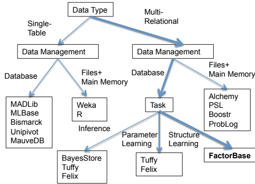
Figure 10. A tree structure for related work in the design space of machine learning \times data management
