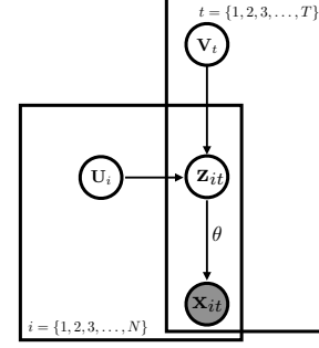
Figure 3. Graphical model of Factorized VAE
