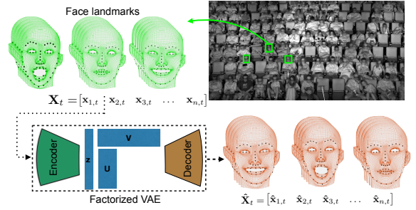
Figure 1. Factorized VAE. Facial landmarks are detected on audience members for the duration of a movie. Tensor factorization assumes a linear decomposition. We propose a non-linear version which learns a variational autoencoder such that the latent space factorizes linearly.
