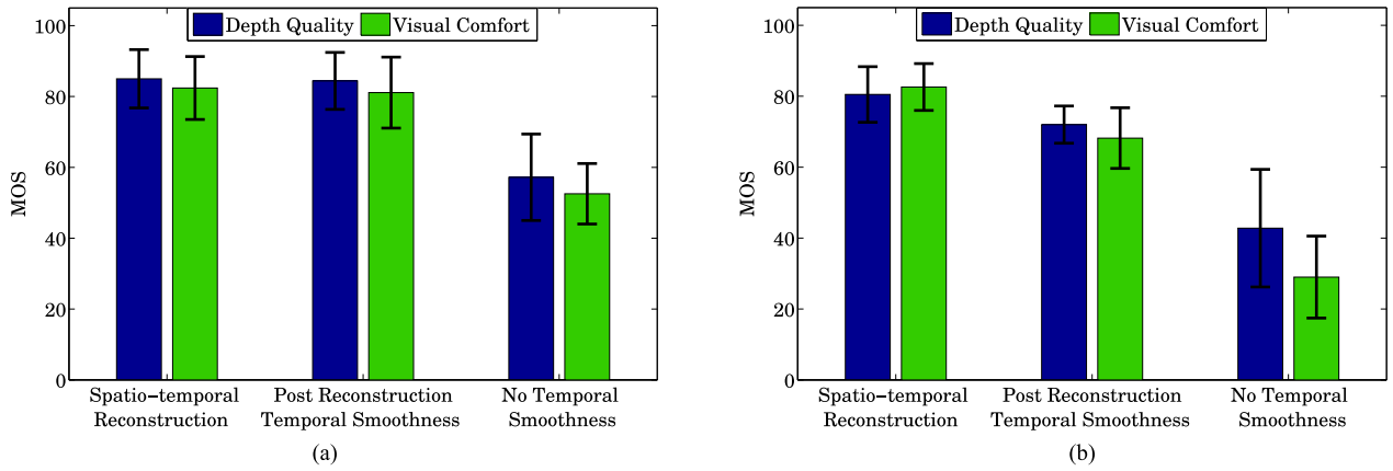
Fig. 14. Mean opinion scores of depth perception and visual comfort for two sequences of different temporal complexity, where three methods are compared: our spatio-temporal Poisson reconstruction, temporal smoothness as a post-process, and without temporal smoothness. (a) Temporally Simple sequence. (b) Temporally Complex sequence.
