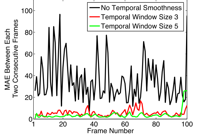
Fig. 18. Mean Absolute Error (MAE) between each two consecutive frames of a real sequence, when using different temporal window sizes.
