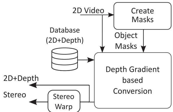
Fig. 1. The proposed 2D-to-3D conversion method.
