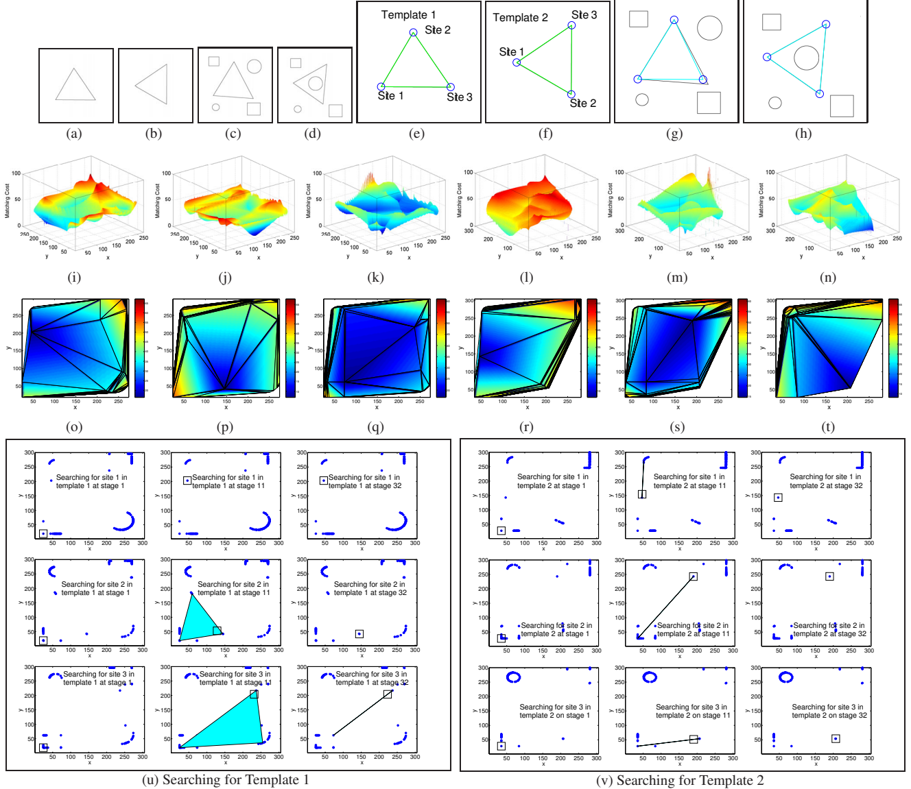
Figure 2. Searching process of the linear program. (a, b) Template images; (c, d) Target images; (e, f) Feature points and template graph; (g, h) Matching result; (i, j, k, l, m, n) Matching cost surfaces for each site on the template; (o, p, q, r, s, t) Convexified matching cost surfaces; (u, v) illustrate the searching process of the linear program.
