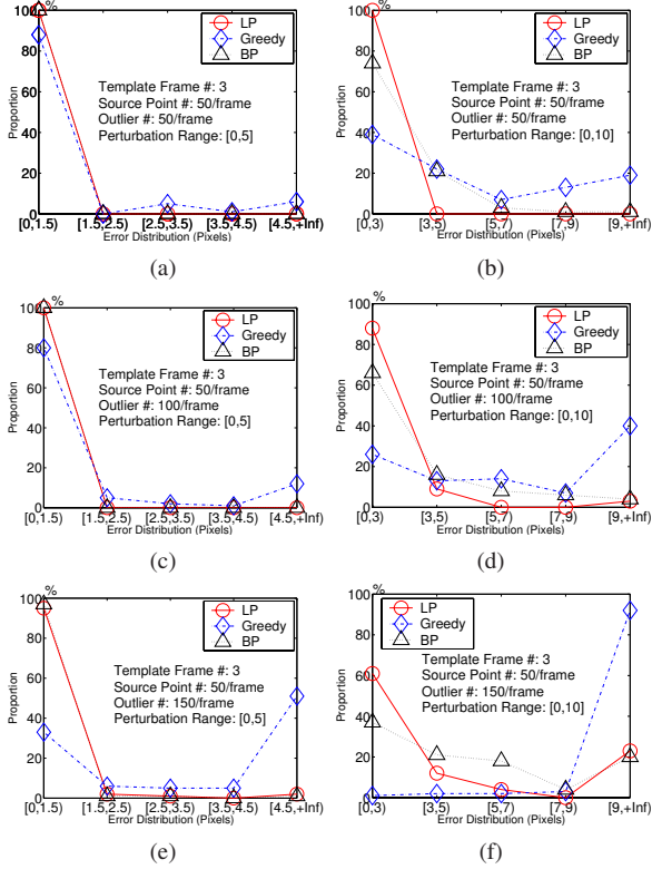
Figure 4. Random sequence matching.
