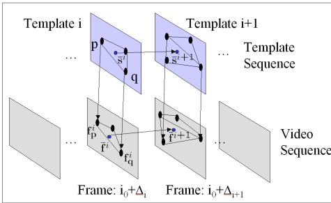
Figure 1. Deformable video matching.
