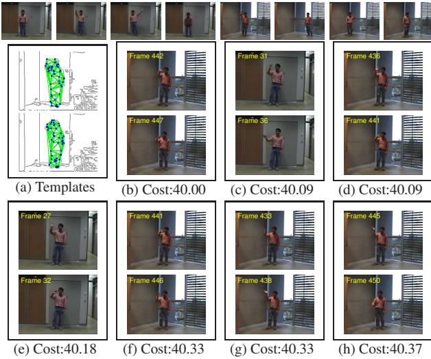
Figure 11. Searching “right hand waving” in a 500-frame indoor sequence. (a) Templates; (b..h) Top 7 matches of the shortlist.
