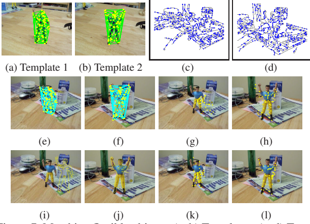
Figure 7. Matching flexible objects. (a, b) Templates; (c, d) Target image edge maps and feature points; (e, f) Matching with the proposed scheme; (g, h) Matching with greedy scheme; (i, j) Chamfer matching for each image pair; (k, l) Matching with BP for each image pair.
