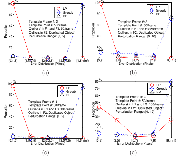
Figure 5. Matching random sequences.
