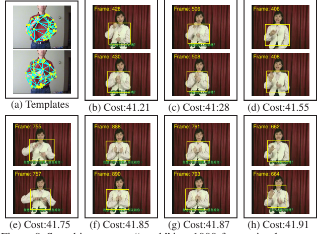
Figure 8. Searching gesture “work” in a 1000-frame sign language sequence. (a) Templates; (b..h) Top 7 matches of the shortlist.
