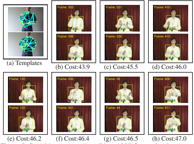
Figure 9. Searching gesture “year” in a 1000-frame sign language sequence. (a) Templates; (b..h) Top 7 matches of the shortlist.
