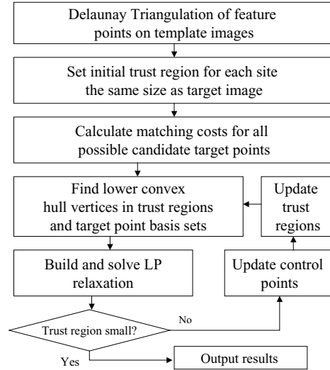
Figure 3. Successive convex matching.
