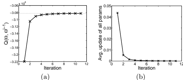
Figure 3: The (a) value of Q(\Theta, \Theta^{(i-1)}) and (b) average difference of all parameters in one iteration.
