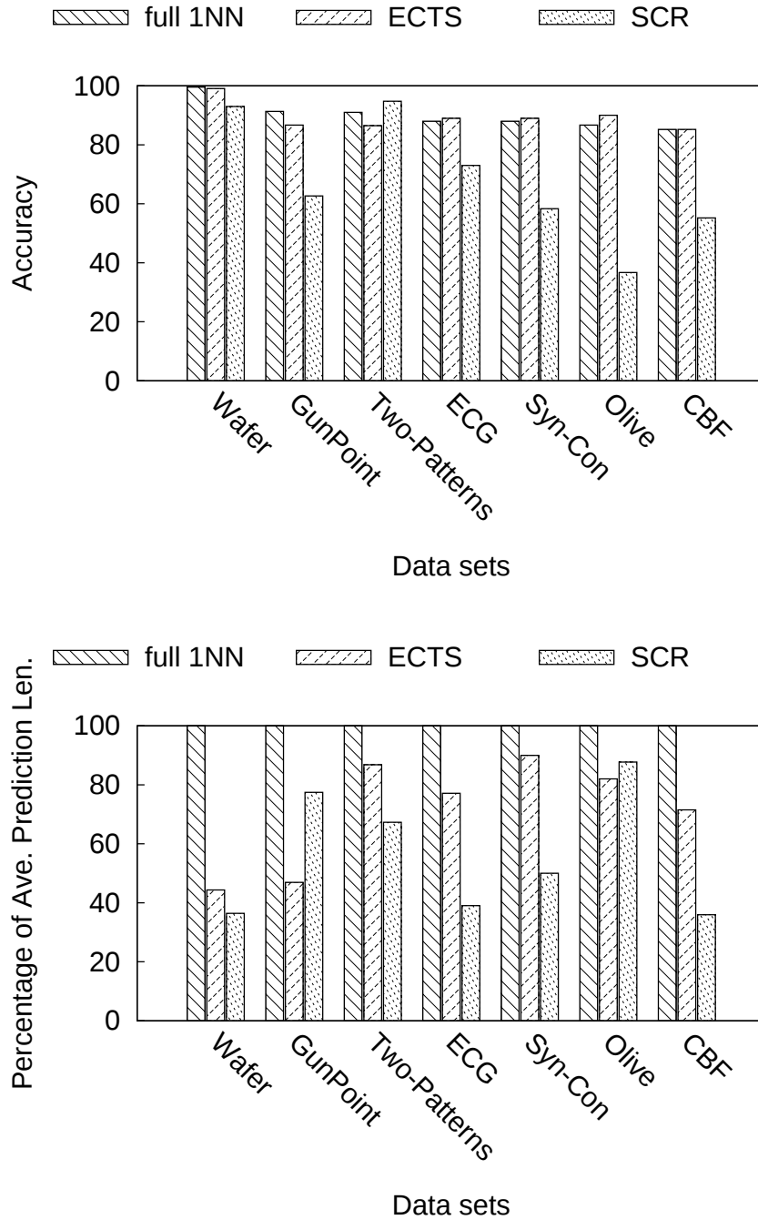
Fig. 6. Comparison between ECTS and SCR. Although SCR sometimes uses a shorter average prediction length, the accuracies are significant lower than the expected values. Comparing to SCR, ECTS makes early classification reliable in accuracy. In terms of efficiency, ECTS is much faster than SCR in training.
