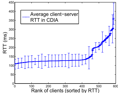
Fig. 4. Average user-server latency in CDIA.
