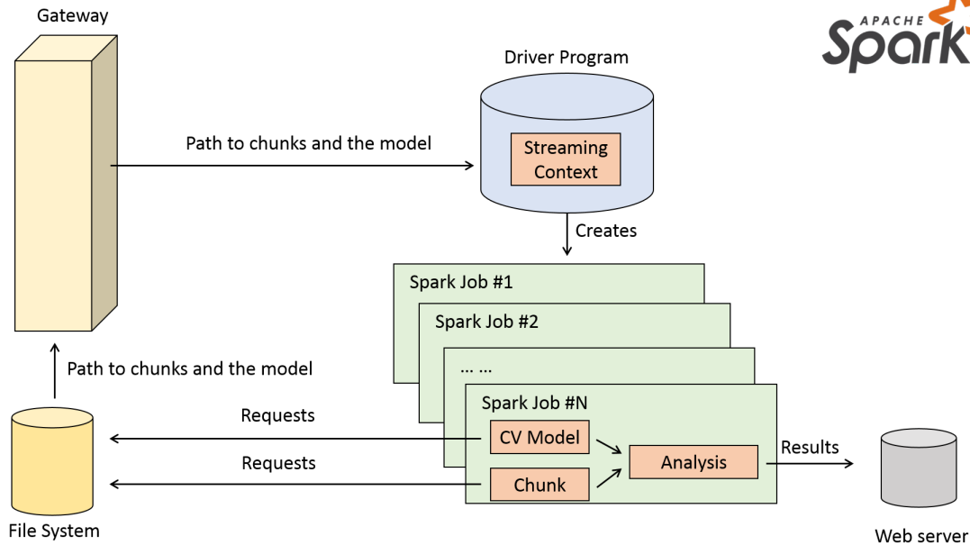
Figure 2: Architecture of the Distributed Video Processor
