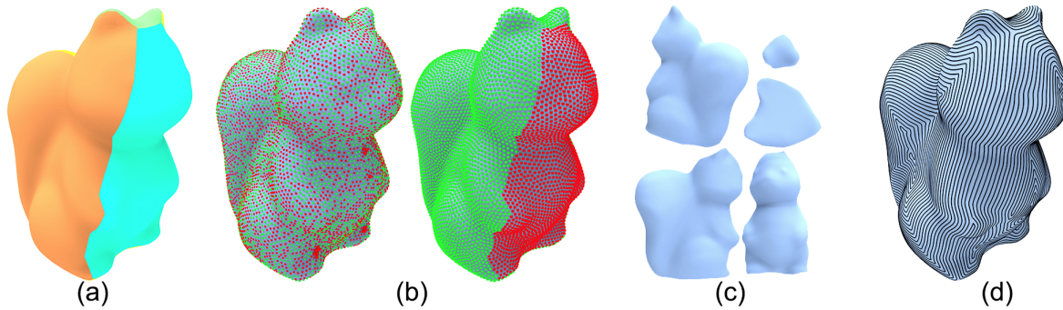
Fig. 2. Overview of DSCarver, our decompose-and-carve algorithm for 3+2-axis CNC machining of freeform 3D objects. (a) Input 3D shape with pre-segmentation into few height fields. (b) Decomposition into accessible regions (left: with overlaps; right: after boundary extraction). (c) Integration of accessibility decomposition (b) and height fields (a) into machinable patches. (d) Connected iso-scallop Fermat spiral paths computed for a few patches.
