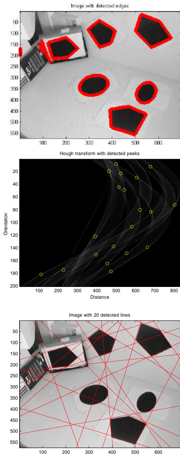
Figure 15: Top; image with detected edges, middle; vote histogram with selected lines, bottom; image with detected lines.
