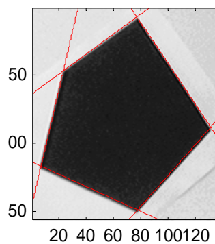
Figure 12: Detected lines.
