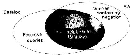
Fig. 2. The expressive power of Datalog.
