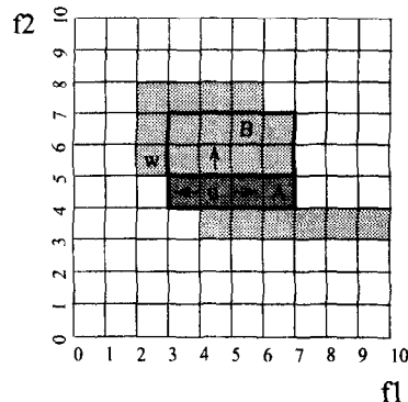
Figure 4: Illustration of the greedy growth algorithm.
