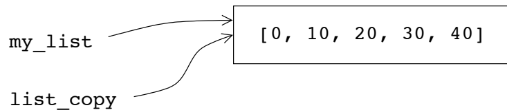
Figure 5.6: Changing either alias changes both
