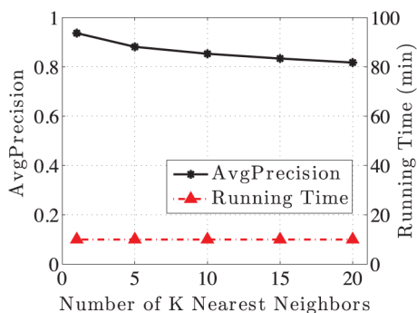
Fig. 7. Effect of K on running time and accuracy.
