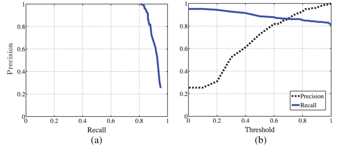
Fig. 3. Performance of the complete system for 3-D video copy protection on more than 11,000 3-D videos. (a) Precision-recall curve. (b) Precision and recall versus threshold s .
