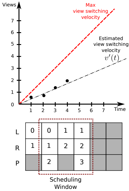
Figure 2: Segment scheduling window. Deciding on left (L) reference view, right (R) reference view, and pre-fetched (P) view.
