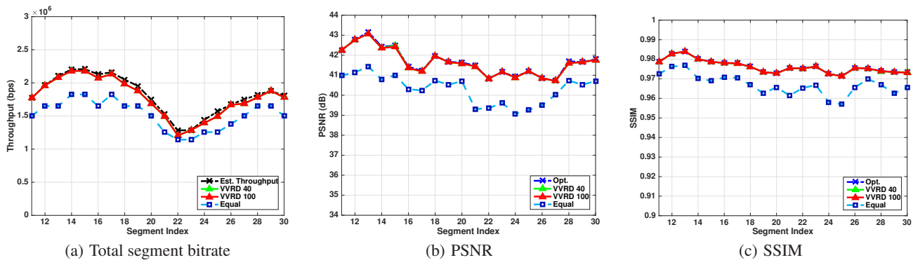
Figure 10: Results for the Kendo video sequence with variable network bandwidth.
