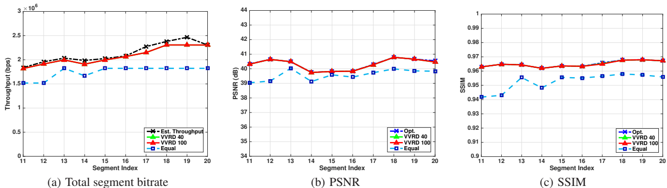
Figure 11: Results for the Café video sequence with variable network bandwidth.
